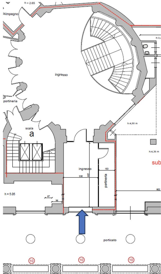
PIANO TERRA
