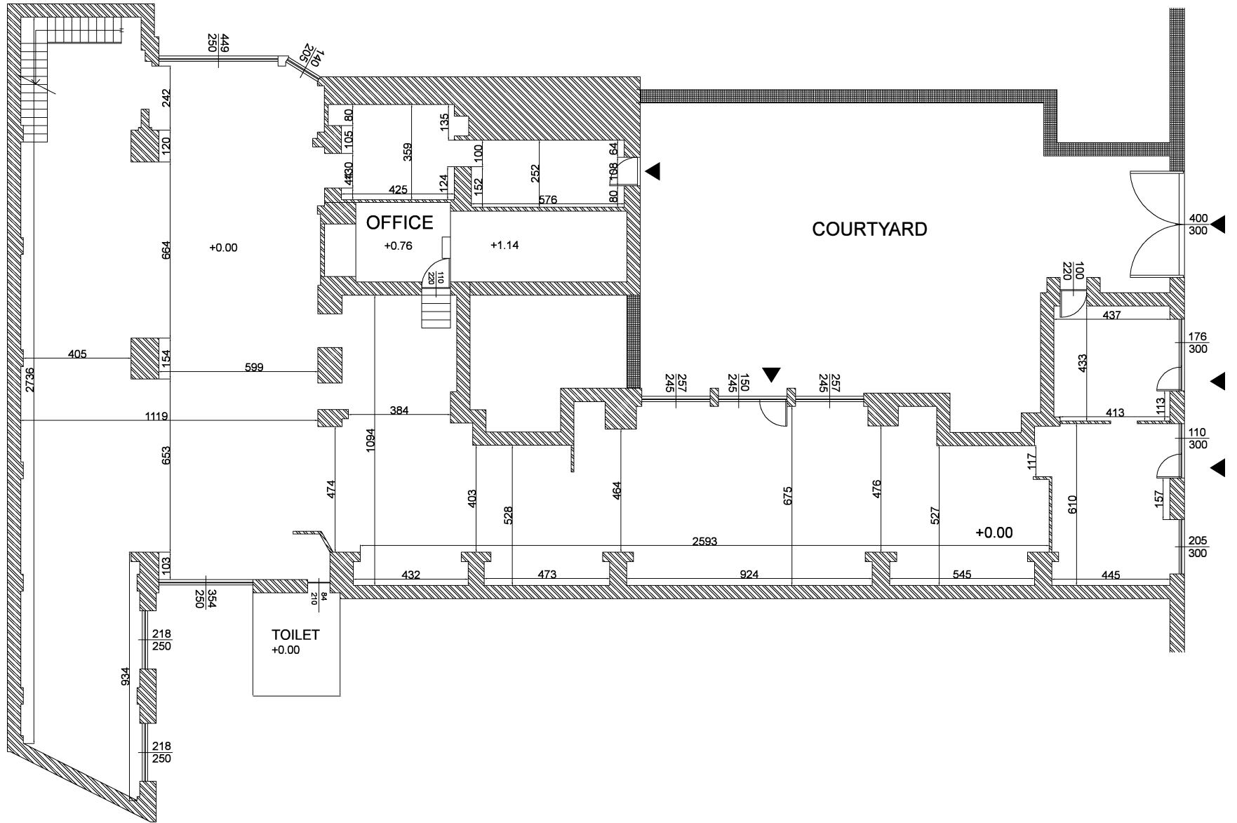
GROUND FLOOR
